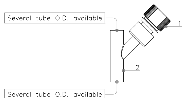
ENFit Y medication port with cap
