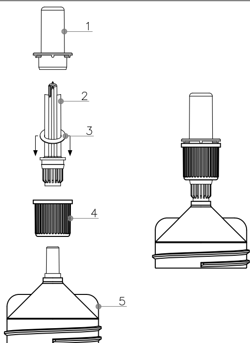
ENPlus screw cap adapter
