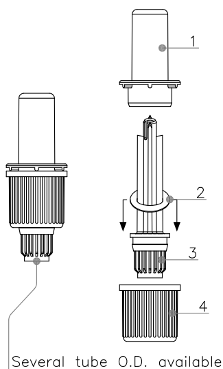
ENPlus cross connector assembly
