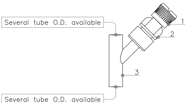
ENFit Y medication port with Oral/Luer adapter and cap
