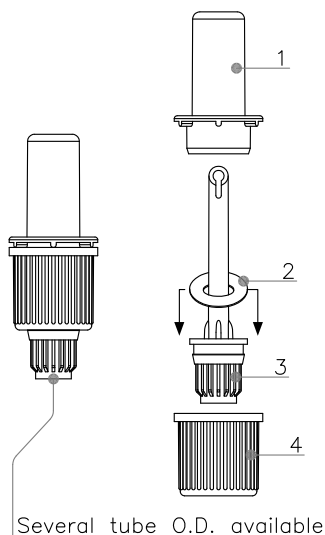
Universal thin connector assembly
