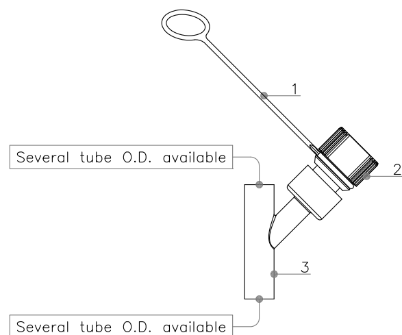
ENFit Y medication port with strap and female cap
